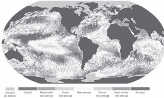
Anomalies and extremes in sea surface temperature in March 2026 Data: ERA5 1979-2026 • Reference period: 1991-2020 • Credit: C3S/ECMWF
